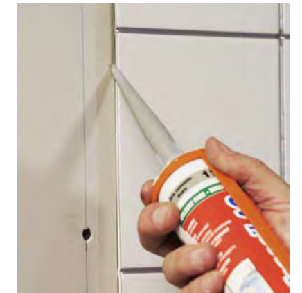
9. Apply small bead of sealant to panel edge.
