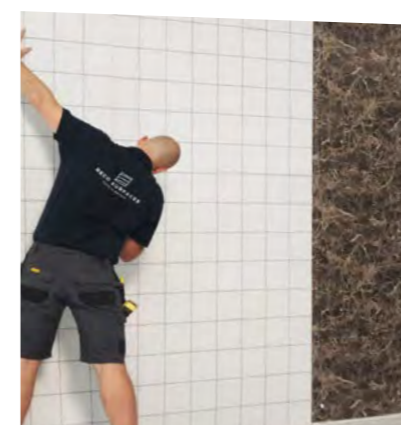
10. Slide second panel up to first allowing 3mm gap between them
