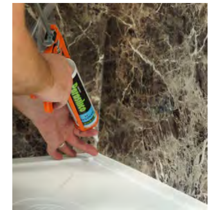
12. Seal top and bottom joints.
